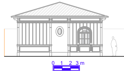
Elevation 03
